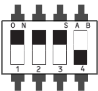
Relais 7
